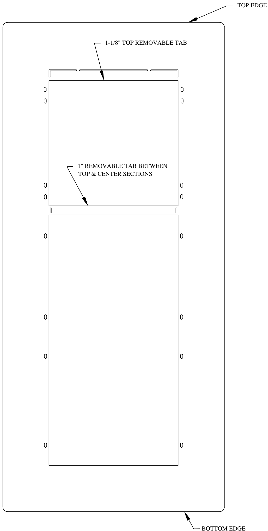
FRONT VIEW
